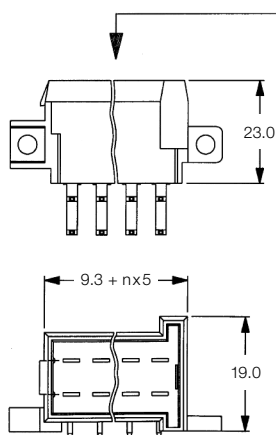
Pin Header 90°
