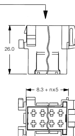
Tab Housing
