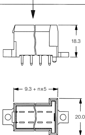
Pin Header 180°
