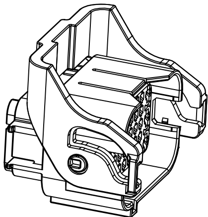
3D-VIEW SCALE 1/1
