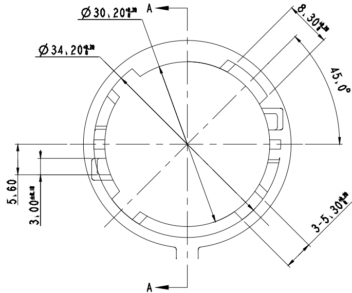
PLUG HOLE(S:2/1)
