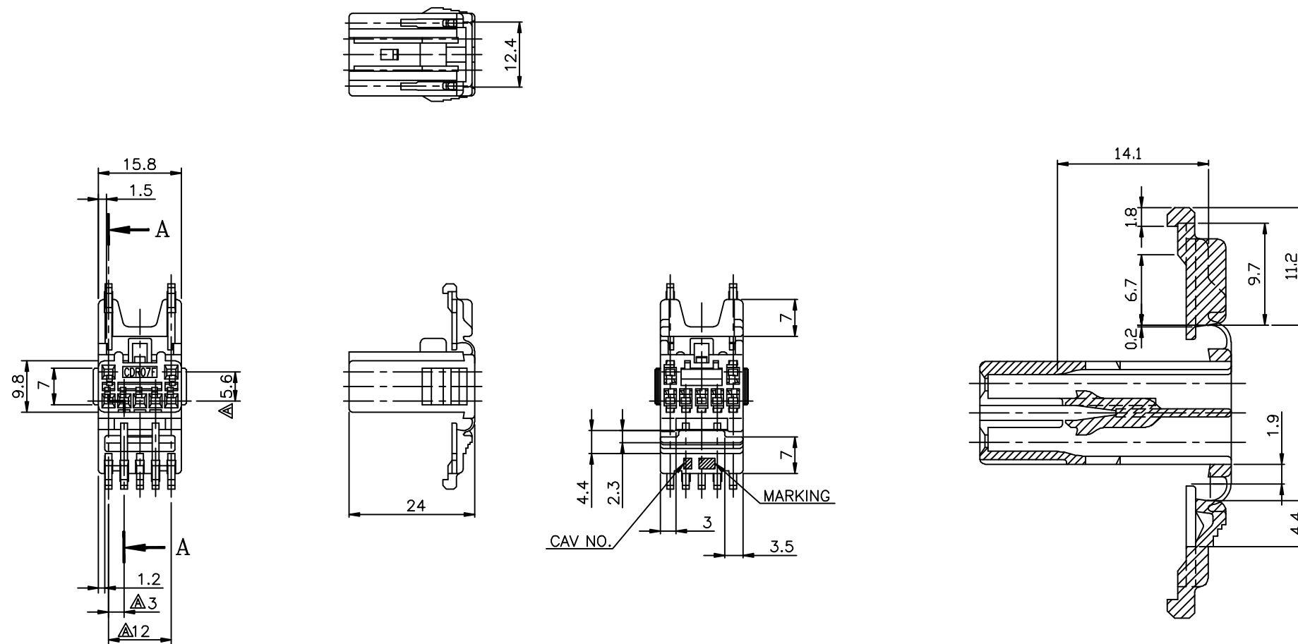
SECTION A-A(2/1)
