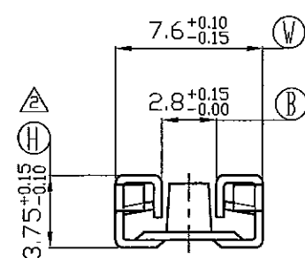
SEC.C-C
